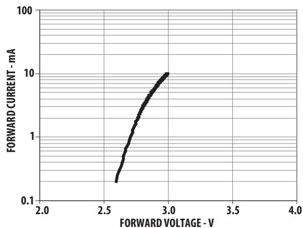
Figure 2. Forward voltage vs. forward current
