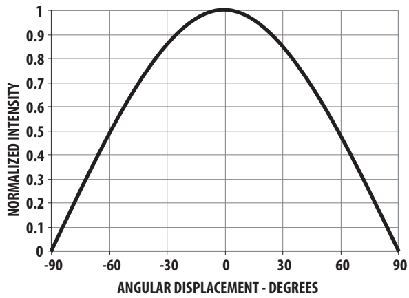
Figure 5. Radiation Pattern
